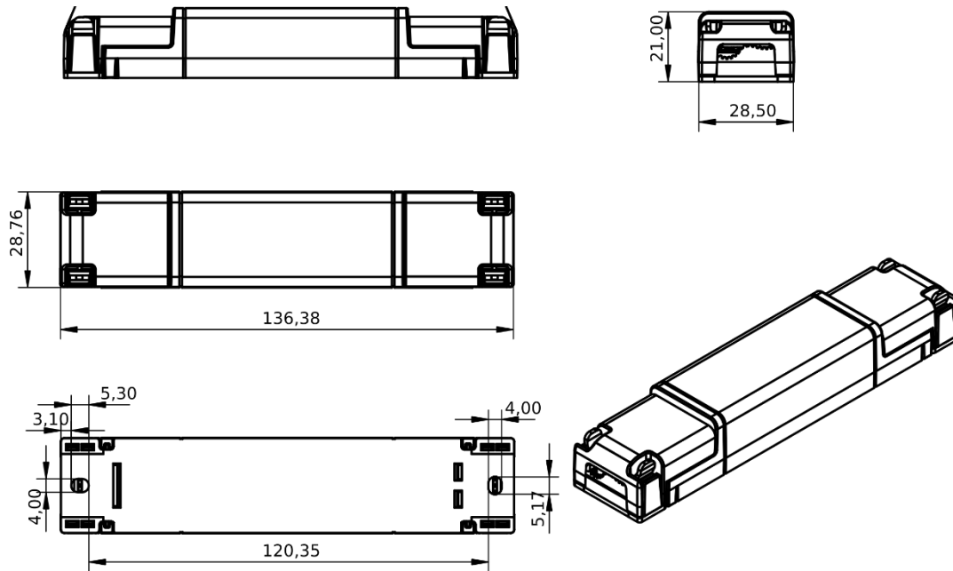
Figure 11: Mechanical dimensions
