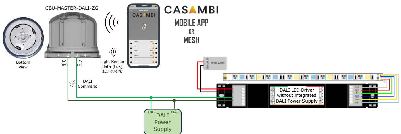
Figure 2: Wiring diagram for LED Driver with external DALI Power Supply
