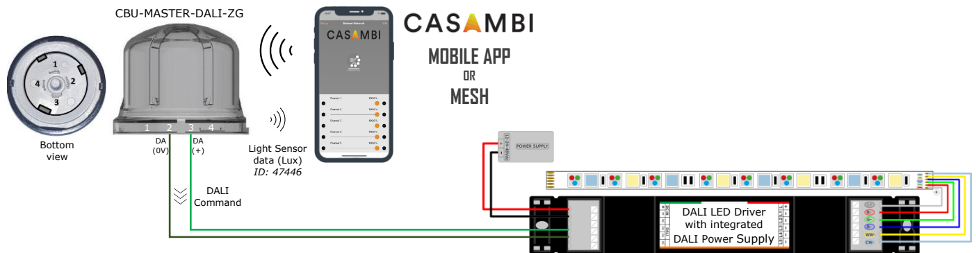
Figure 1: Wiring diagram for LED Driver with integrated DALI Power Supply
