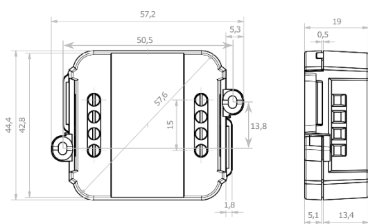
DLM1224-1CV Variant
