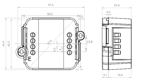
DLM1248-1CV Variant
