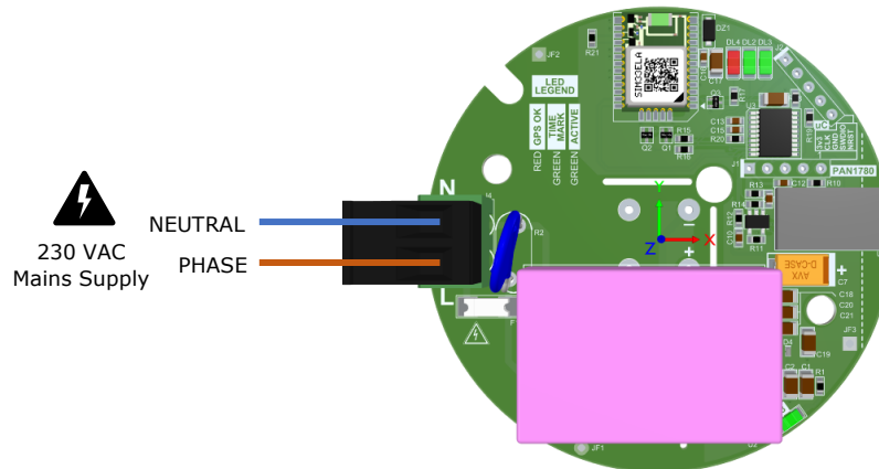
Figure 1: CBU-SKYTIME-IP Power Supply wiring
