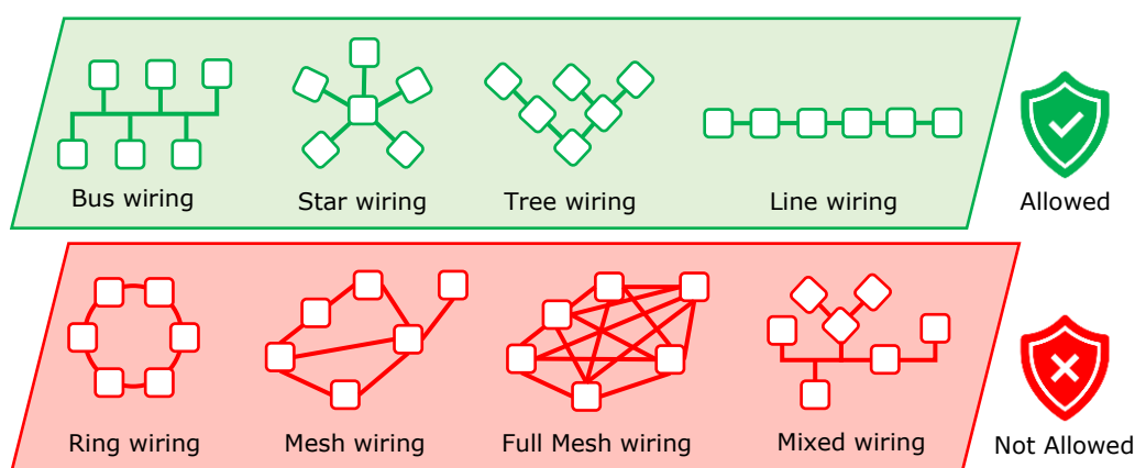
Figure 3: DALI wiring Topologies
