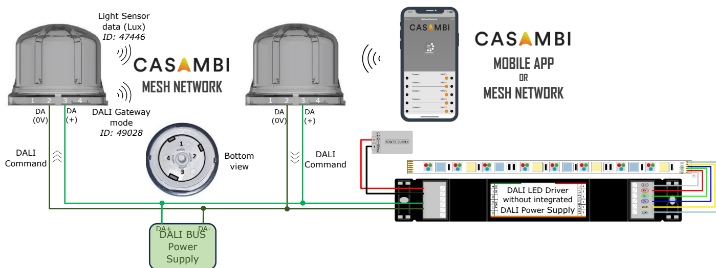
Figure 2: Wiring diagram for LED Driver with external DALI Power Supply
