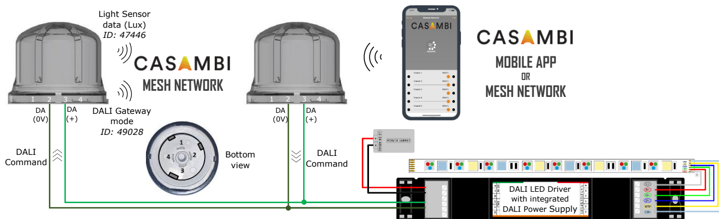
Figure 1: Wiring diagram for LED Driver with integrated DALI Power Supply
